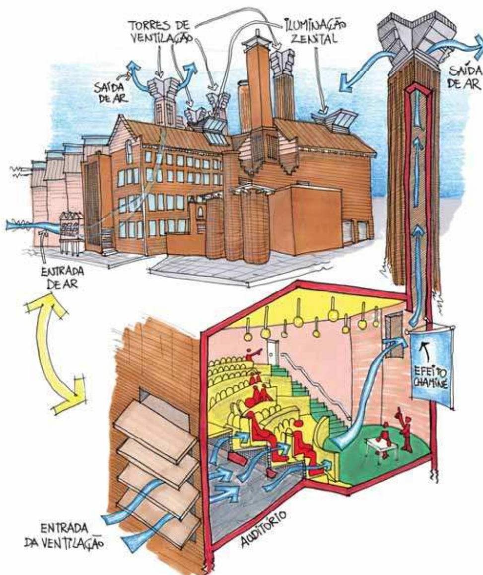
Figura 1-29: Queen's Building
