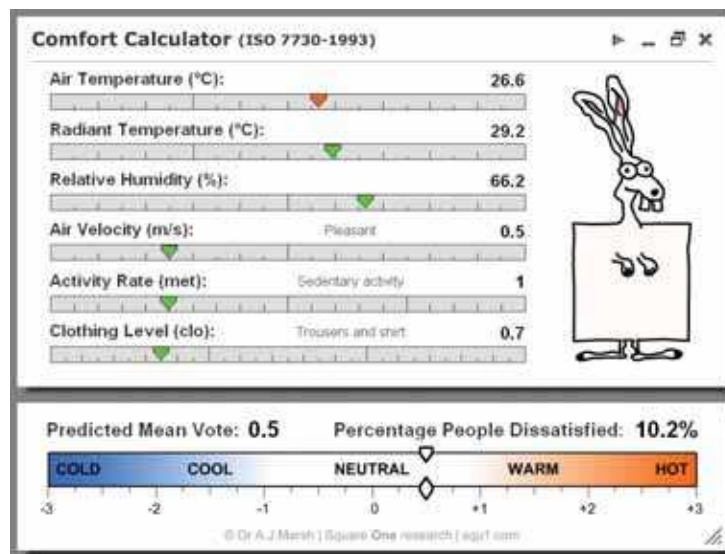
Figura 2-15: Comfort Calculator
