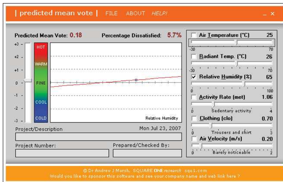
Figura 2-16: PMVTool
